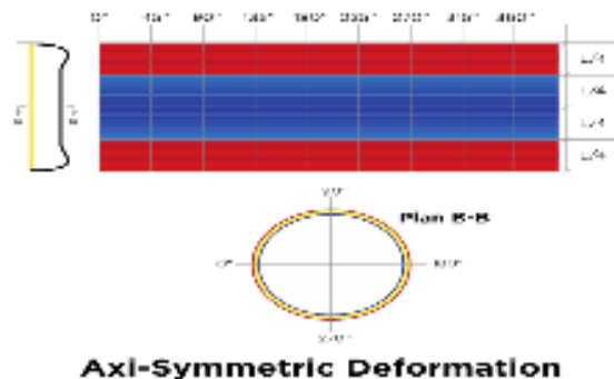
Fig. 9. Axi- symmetric deformation pattern
