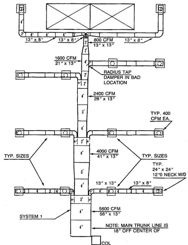
Fig. 3 Typical Airduct System
