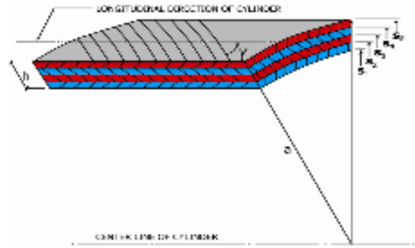
Fig. 6. A laminated cylindrical shell, material orientation
