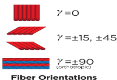
Fig. 5. Fiber orientation
