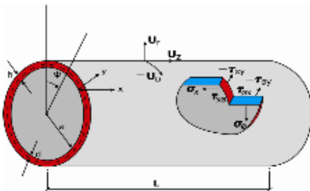
Fig. 4. Dimensions, deformations and stresses of a cylindrical shell
