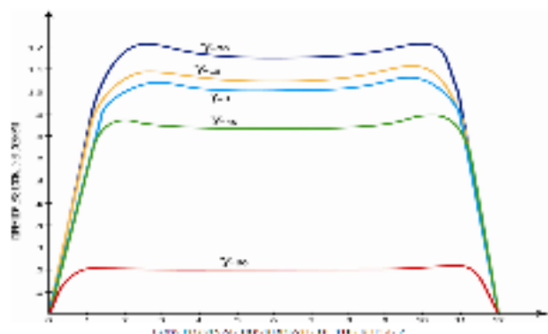
Fig. 8. Radial displacement of theory (ah)^{1/2} with different material angle of orientation single layer
