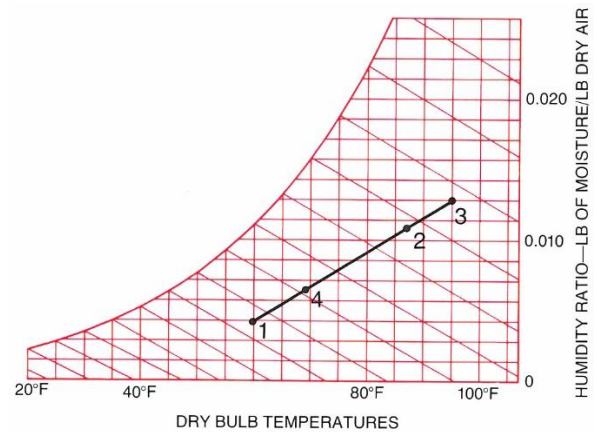
Fig. 2 Psychrometric Chart
